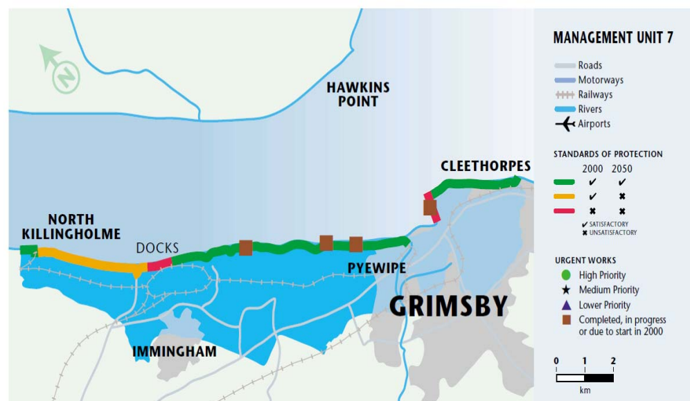
Figure 6.11 Flood Defences in Shoreline Management Plan Unit 7
