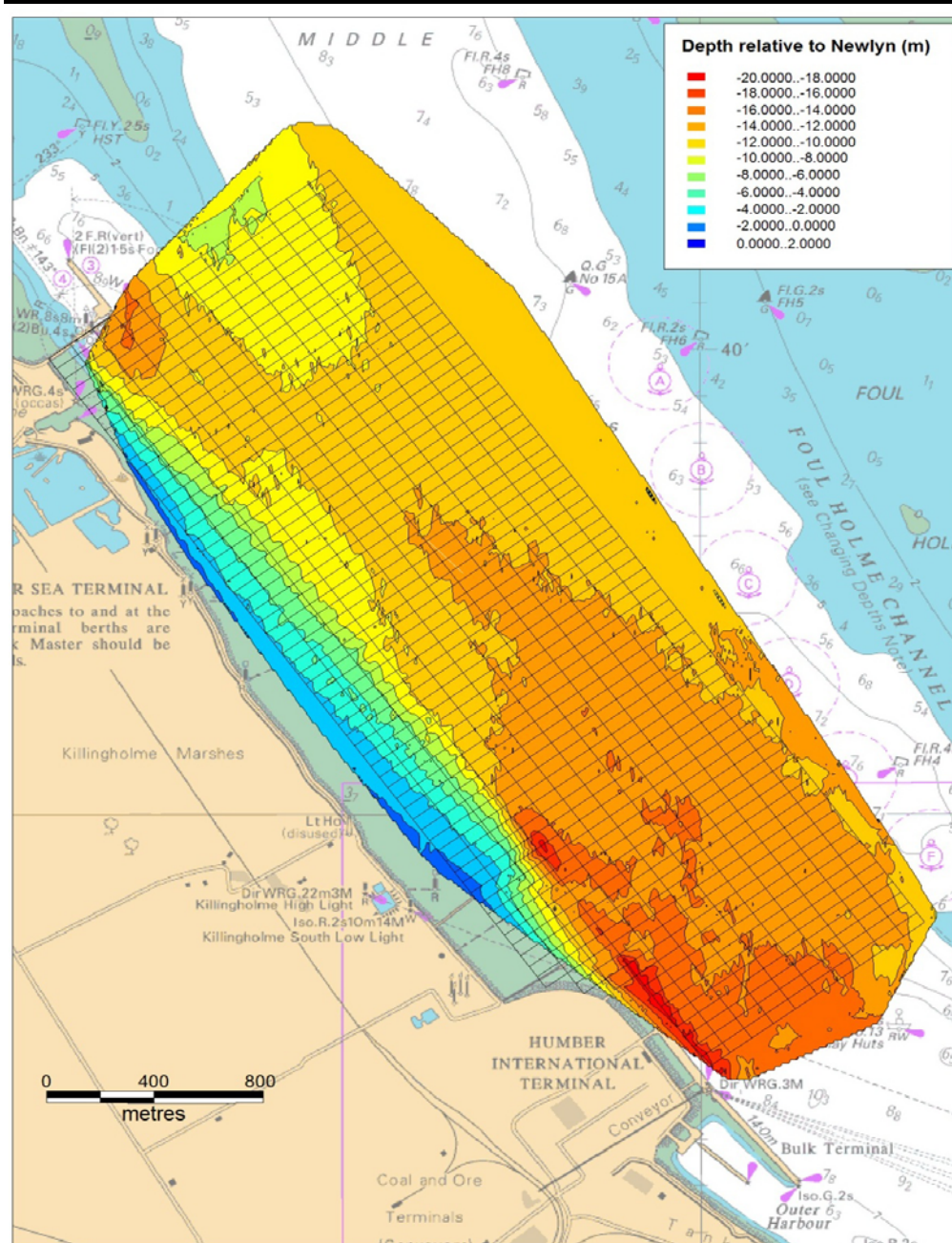
Figure 6.1 Humber Estuary Bathymetry
